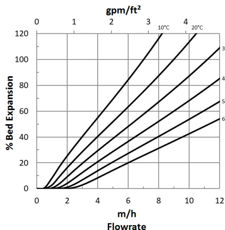
Figure 1: Backwash Expansion
